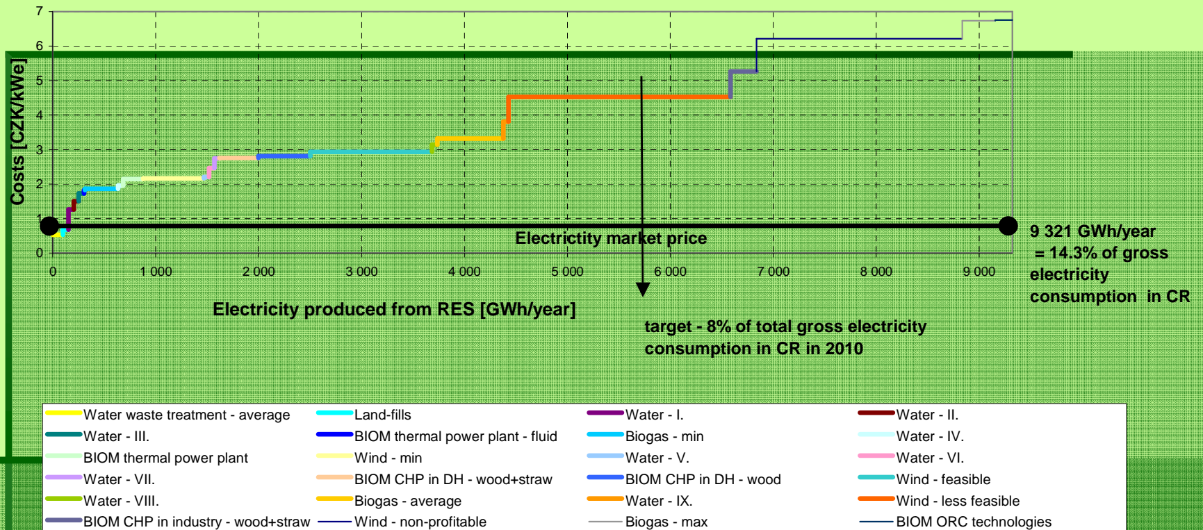
Potential of the Electricity Production from RES - Costs up to 7 CZK/kWh
